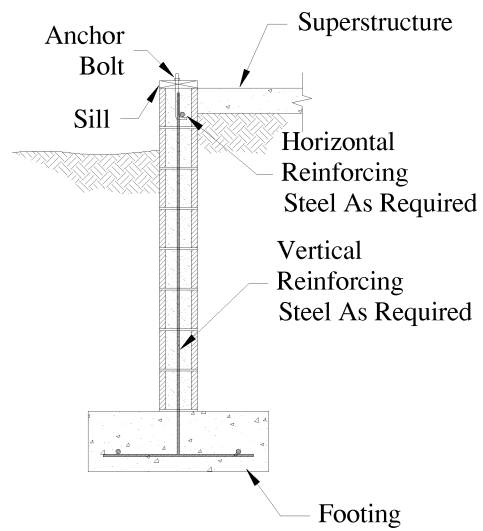
Figure 2-2c: Stem Wall
