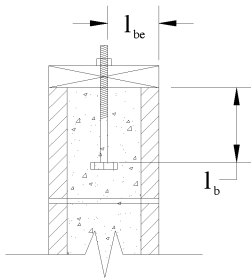
Figure 2-13b: Anchor Dimensioning
