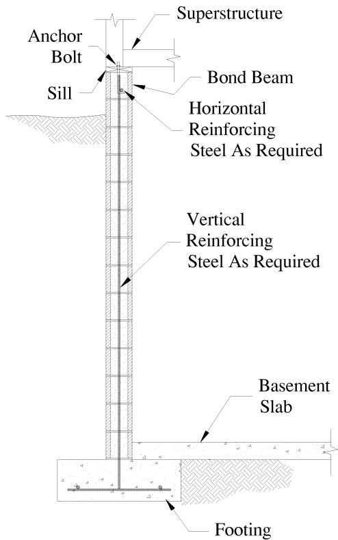
Figure 2-2a: Basement Wall
